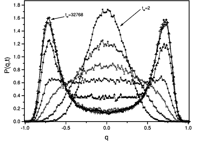
FIG. 13. Overlap distribution P(q, t) vs q , for a system with N = 128 and \alpha = 1 . The different curves correspond to the following times: 2, 4, 8, 16, 64, 512, 4096, 32 768. A total of 15 replicas were used in each of 744 runs with different realizations of the random patterns and thermal noise.
